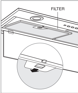
Filter removal (30" model shown)
