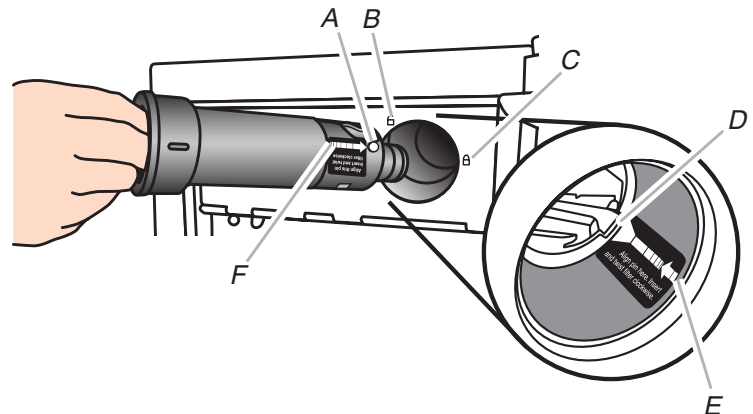
A. Alignment pin B. Unlocked symbol C. Locked symbol
