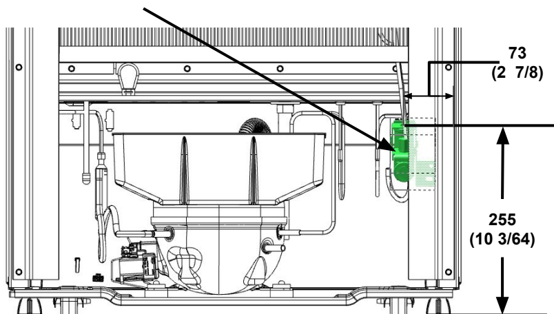
Water valve
