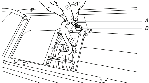
A. Blower motor wire B. Connector
