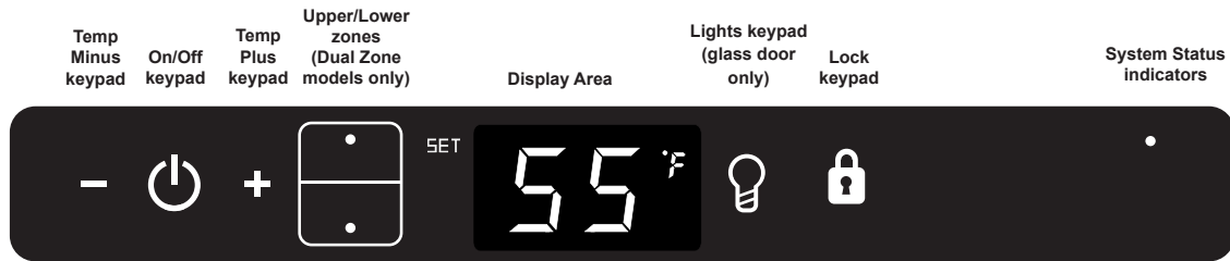
Figure 10 Electronic control
