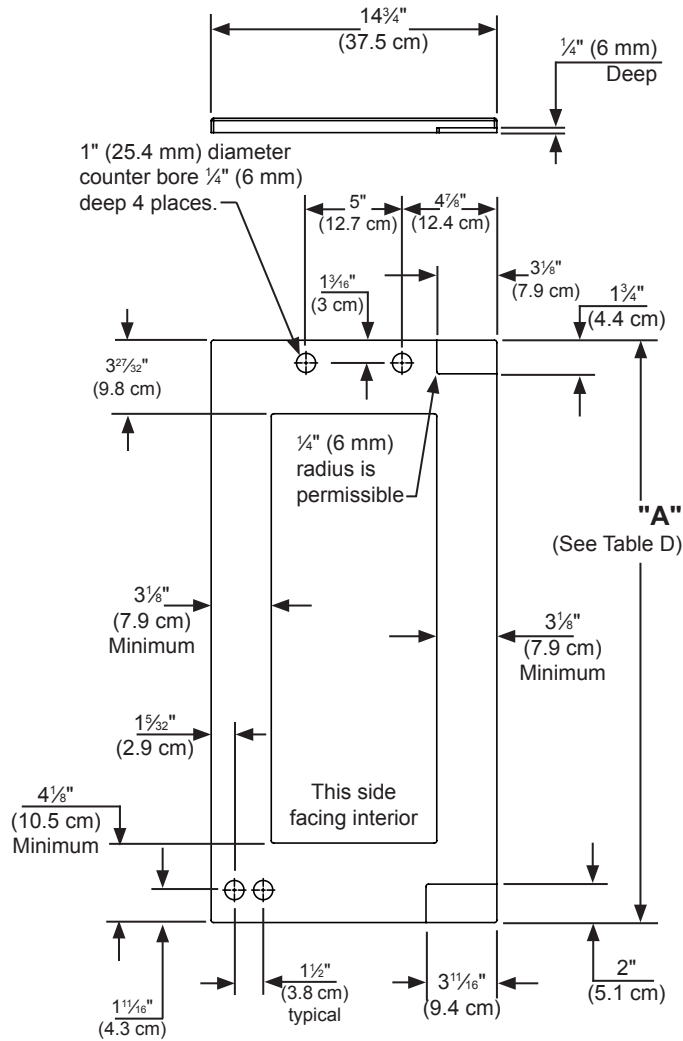
Figure 14 Left Hand Hinged Door 15" (38.1 cm) Wide Appliance
