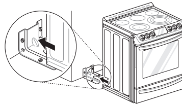
Engage the anti-tip device
