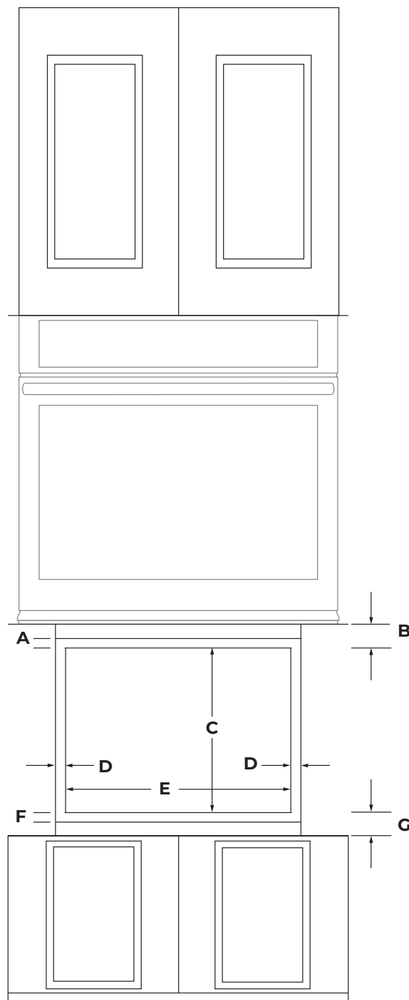
FRONT VIEW
