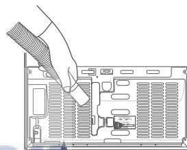
Fig.30 Cleaning the rear compartment cover
