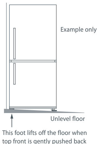
Fig.14 Unstable refrigerator
