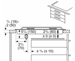
Measurements in inches (mm) Cooktop over drawer
