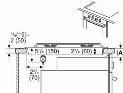
Measurements in inches (mm) Cooktop over oven
