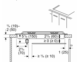
Measurements in inches (mm) Cooktop over door
