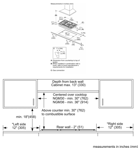
Measurements in inches (mm) Cooktop over oven
