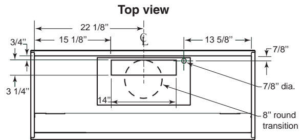
MODEL PIK45 WITH P8 BLOWER (Vertical Outlet)
