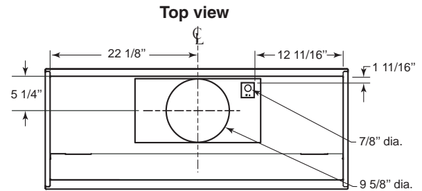
MODEL PIK45 WITH EB6, EB9, EB12 OR EB15 BLOWER (Vertical Outlet)
