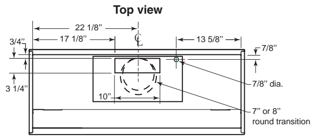
MODEL PIK45 WITH P5 BLOWER (Vertical Outlet)
