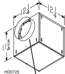
8" ROUND DUCT CONNECTOR
